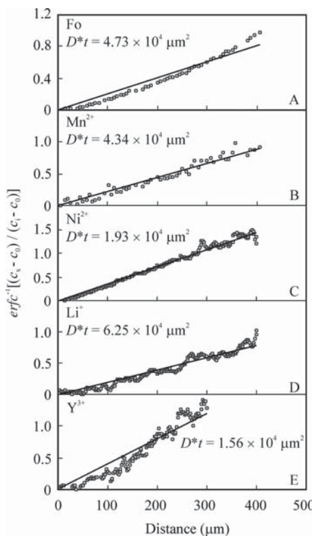
Figure 3. Plots of \text{erfc}^{-1}\left(\frac{c(x) - c_0}{c_1 - c_0}\right) versus distance ( x ) from olivine-melt interface for Fo (i.e., Mg-Fe interdiffusion), Mn, Ni, Li, and Y (see Eq. 1), from top half of traverse b1 shown in Figure 1A. Deviation from a straight line for Fo data is expected from dependence of interdiffusion coefficient D_{\text{Mg-Fe}} on Fo (Dohmen and Chakraborty, 2007). Mg, Fe, and Mn were analyzed by electron microprobe (EMP); other elements were analyzed by laser-ablation-inductively coupled plasma-mass spectroscopy (LA-ICP-MS) by scanning with rectangular beam.
