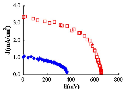
FIG. 2. (Color online) I - V performance of the electrode with (□) or without (◆) DTL based on the 120 mesh net substrate and an 8 \mu\text{m} thick PTL-AM1.5, 100 \text{ mW/cm}^2 .
