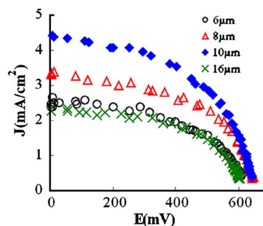
FIG. 3. (Color online) I - V performance of the electrode with different thicknesses of \text{TiO}_2 . AM1.5, 100 \text{ mW/cm}^2 .
